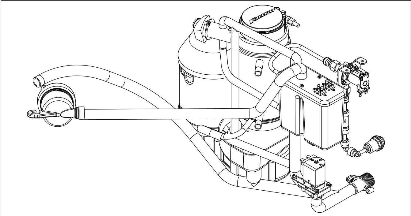
Fig. 19 - Water Reservoir
