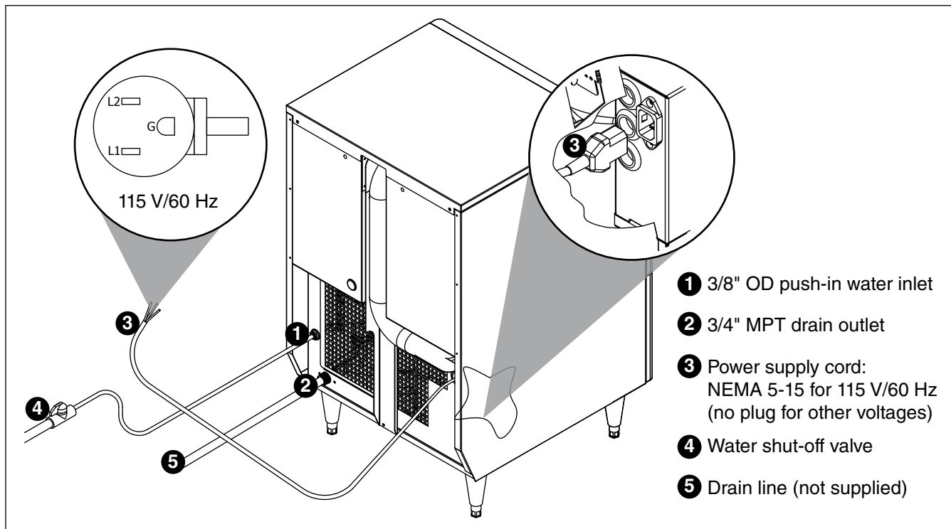
Fig. 6 - Freestanding
