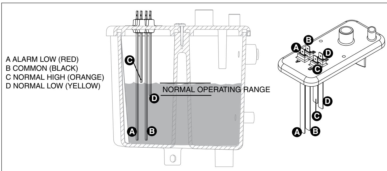
Fig. 19 - Water Reservoir
