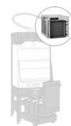
RIDE model
