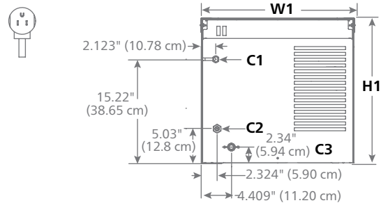
C1 Back view — water-cooled, top mount
