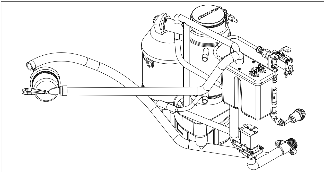
Fig. 18 - Water Reservoir
