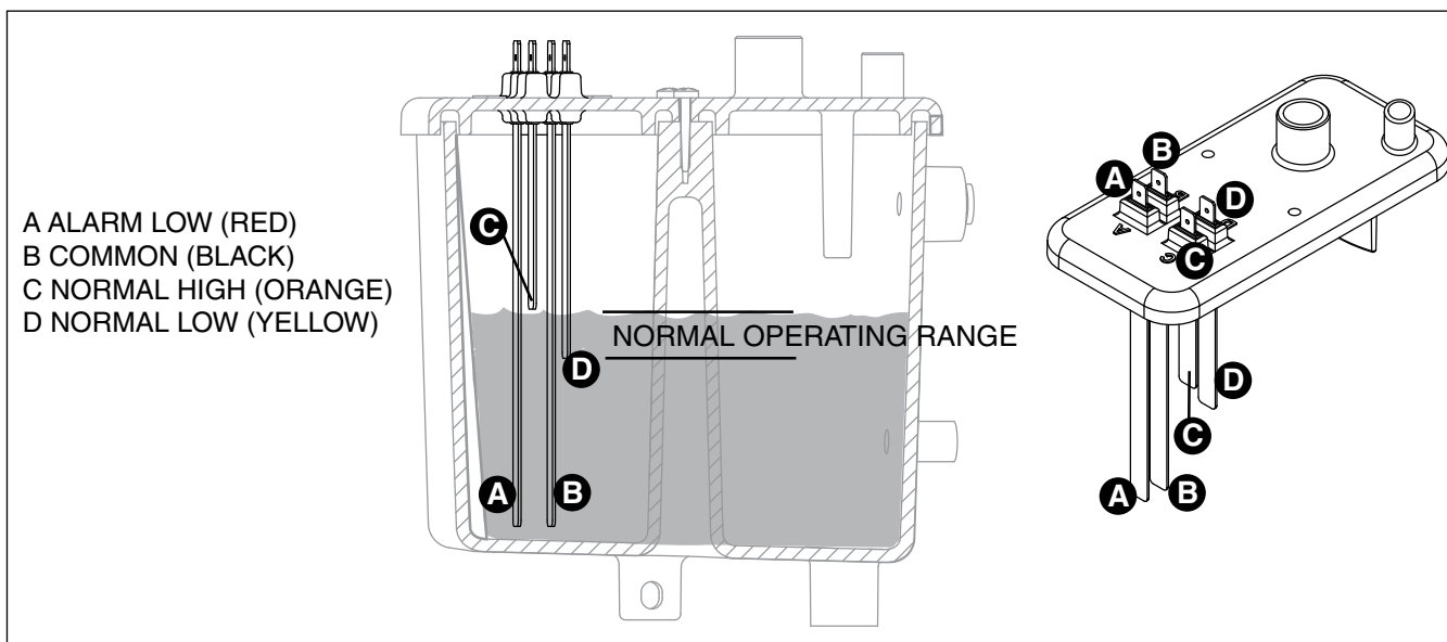
Fig. 18 - Water Reservoir
